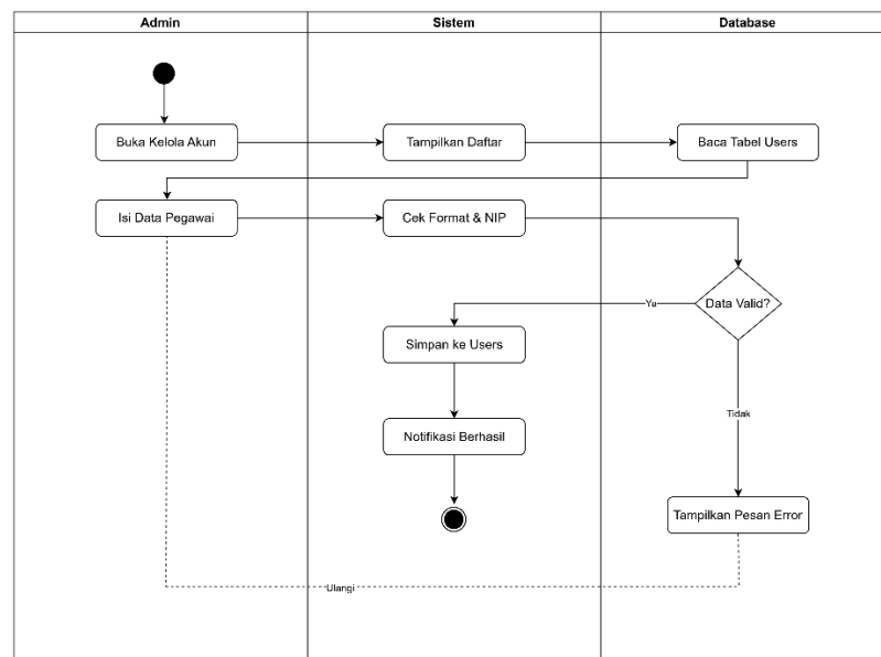
Gambar 3.5 Activity Diagram Kelola akun Pegawai
