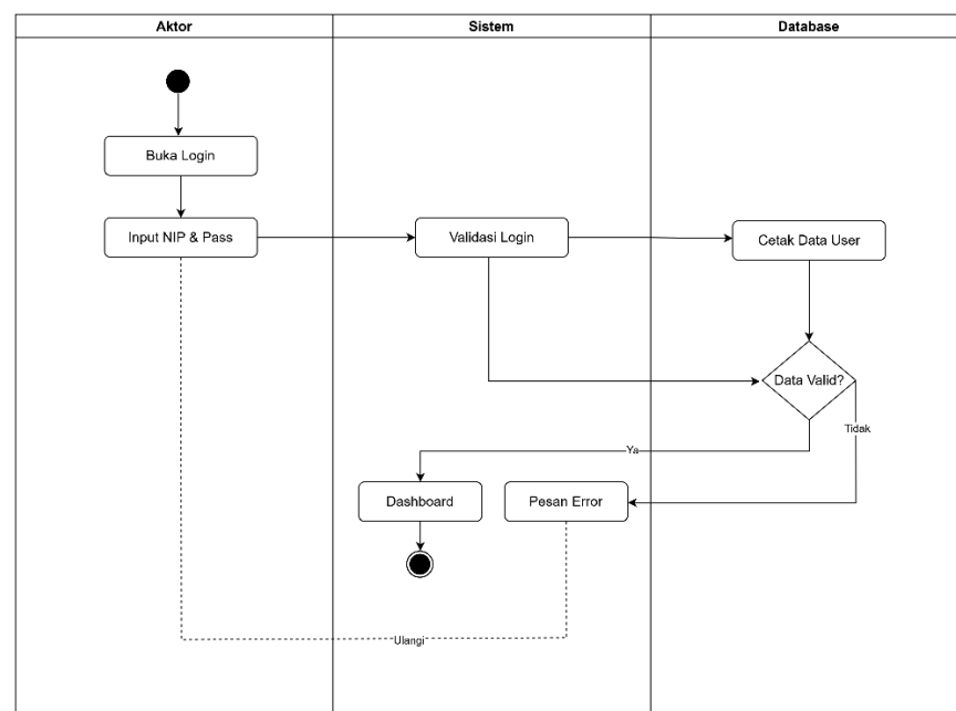
Gambar 3.4 Activity Diagram Login
