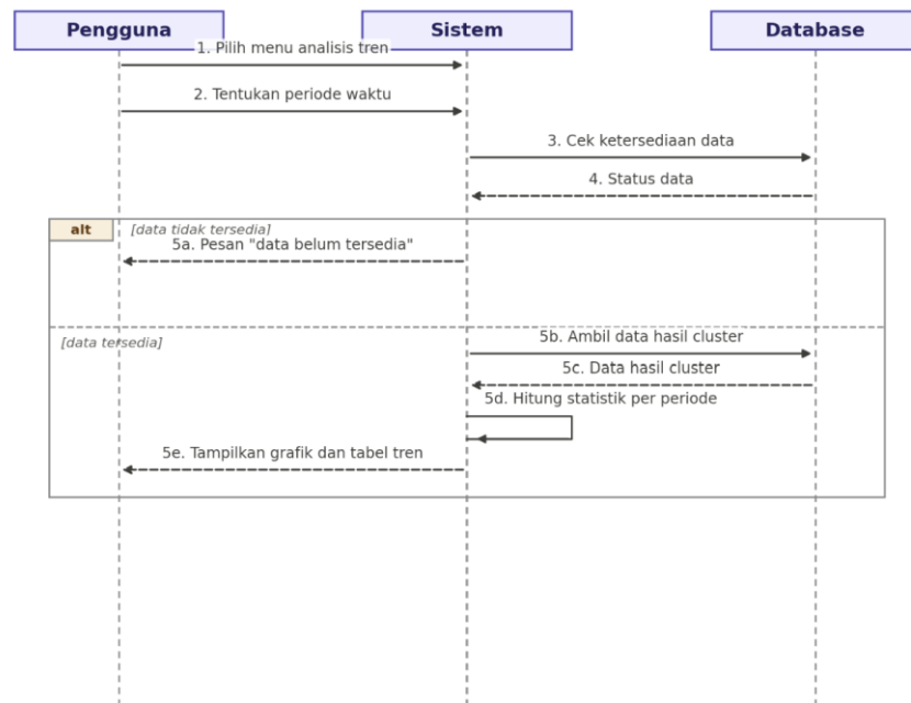
Gambar 3.11 Sequence Diagram Analisis Tren
