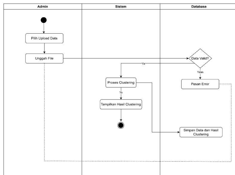
Gambar 3.6 Activity Diagram Clustering
