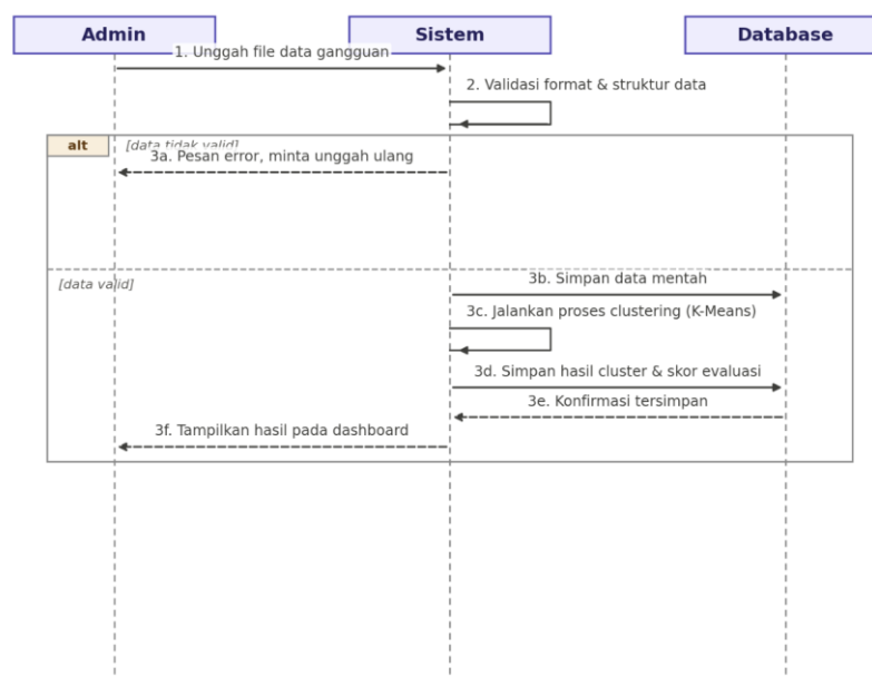
Gambar 3.10 Sequence Diagram Clustering
