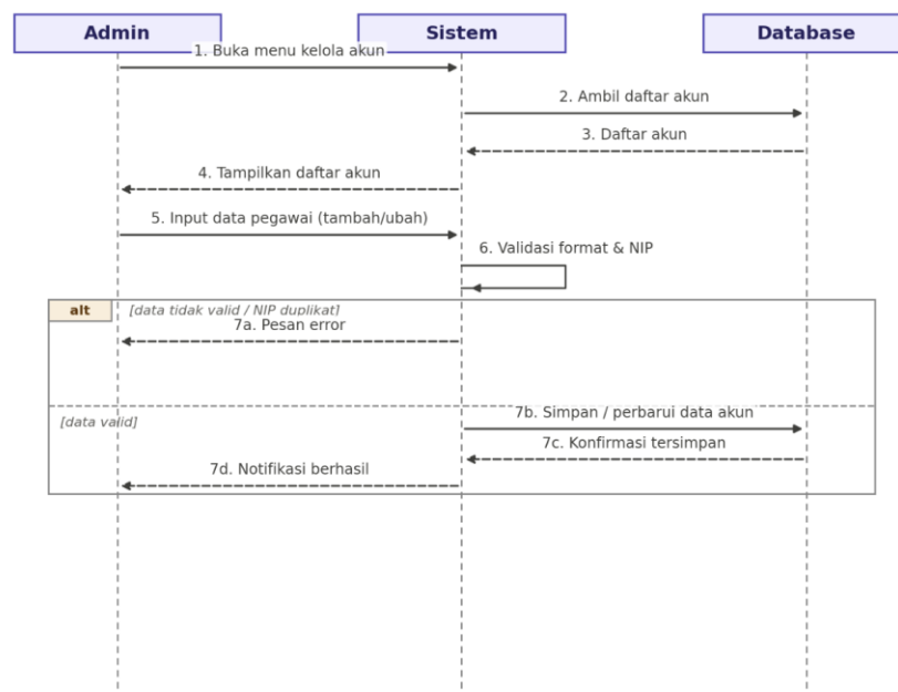
Gambar 3.9 Sequence Diagram Kelola Akun
